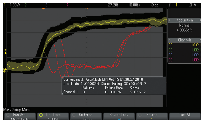
Figure 6: Mask testing to 6.2 s resolution takes only seconds using an InfiniiVision scope with a mask test rate of 270,000 waveform tests per second
