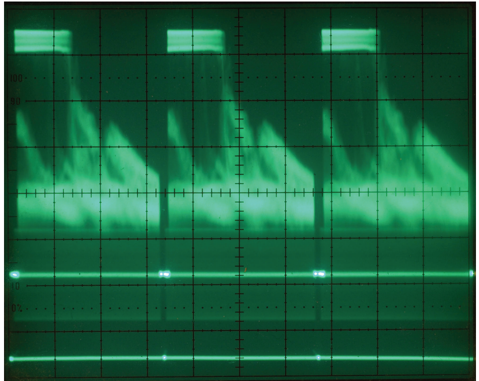
Figure 1. Full frame of composite video displayed on a 100-MHz analog oscilloscope.
