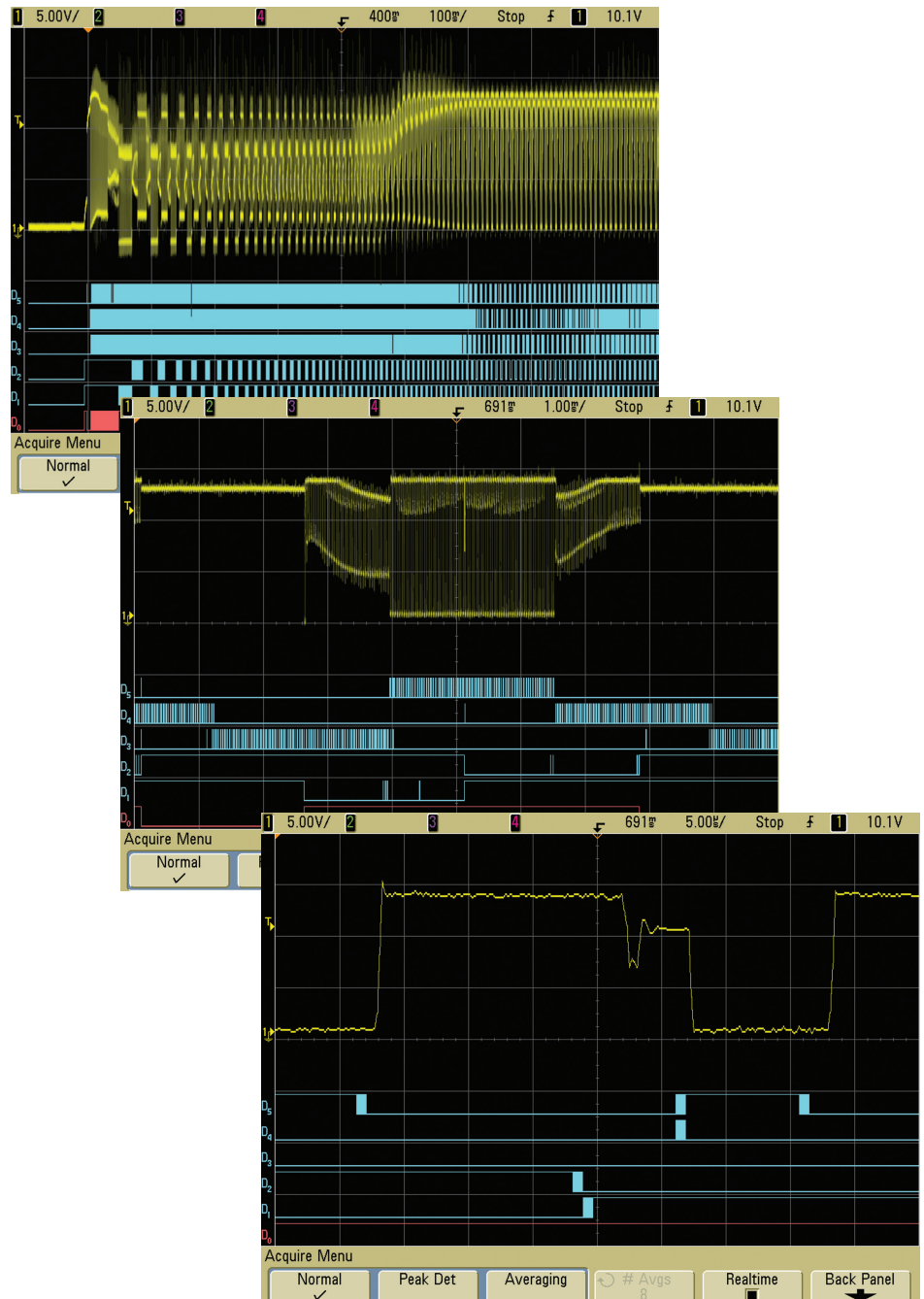
Figure 5. Motor drive signal start-up sequence with digital control signal triggering and various levels of zoom to reveal a "runt" pulse using a Keysight InfiniiVision Series MSO.
