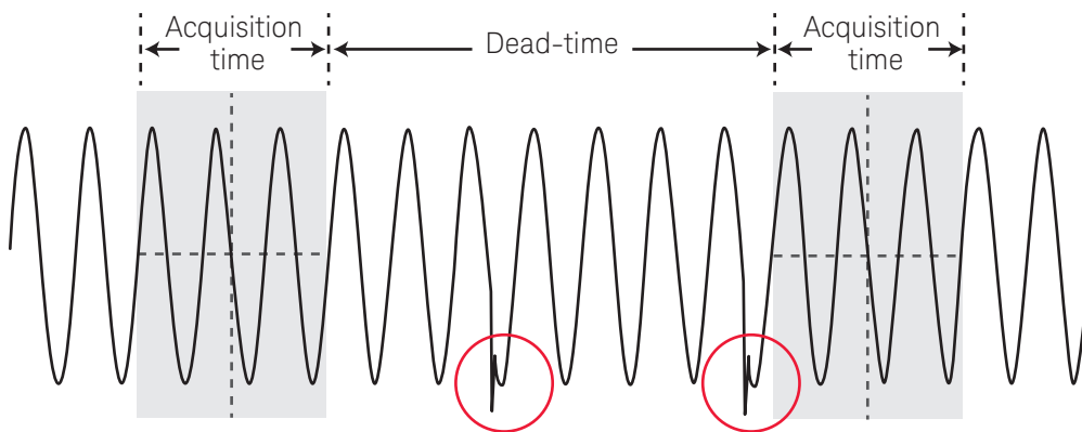
Figure 1. Oscilloscope dead-time versus display acquisition time.
