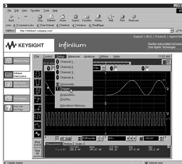
Figure 7. The virtual front panel of the Infiniium oscilloscope enables browser-based interaction with the instrument.
