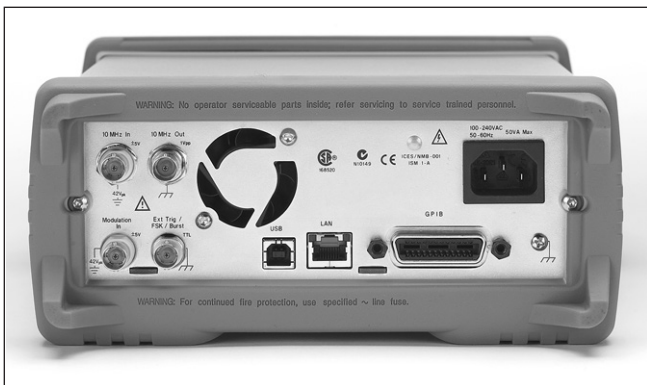
Figure 5 The rear panel of the 33220A function generator includes USB, LAN and GPIB interfaces.
