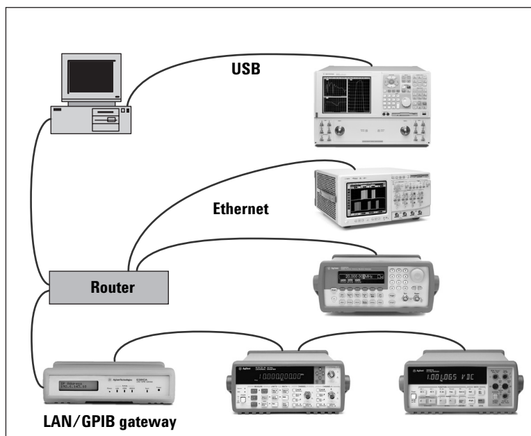
Figure 4 An example test system that utilizes a PC, several instruments, a LAN router, a LAN/GPIB gateway and three types of I/O.
