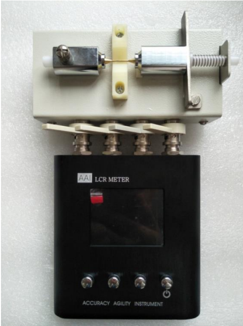
Figure 5-1 Thimble type test stand
