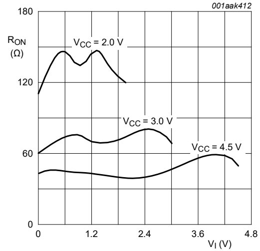
Fig. 10. Typical RON as a function of input voltage
