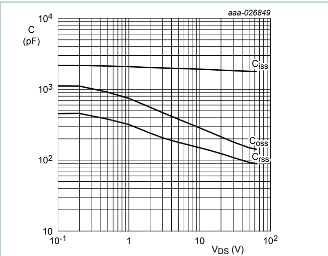
V_{GS} = 0 V; f = 1 MHz Fig. 15. Input, output and reverse transfer capacitances as a function of drain-source voltage; typical values, FET1 and FET2
