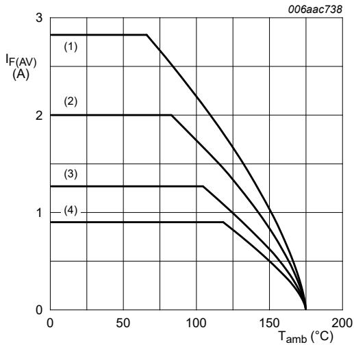
FR4 PCB, mounting pad for cathode 1 cm 2 T_j = 175\text{ °C} (1) \delta = 1.0 (DC) (2) \delta = 0.5 ; f = 20\text{ kHz} (3) \delta = 0.2 ; f = 20\text{ kHz} (4) \delta = 0.1 ; f = 20\text{ kHz}
