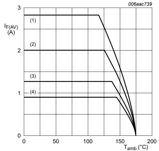
Ceramic PCB, Al 2 O 3 , standard footprint T_j = 175\text{ °C} (1) \delta = 1.0 (DC) (2) \delta = 0.5 ; f = 20\text{ kHz} (3) \delta = 0.2 ; f = 20\text{ kHz} (4) \delta = 0.1 ; f = 20\text{ kHz}
