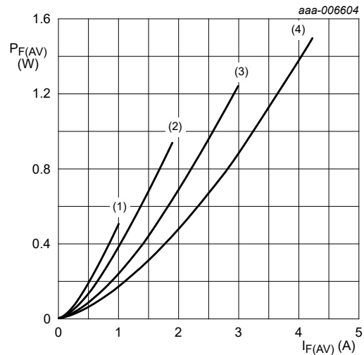
T_j = 175\text{ °C} (1) \delta = 0.1 (2) \delta = 0.2 (3) \delta = 0.5 (4) \delta = 1
