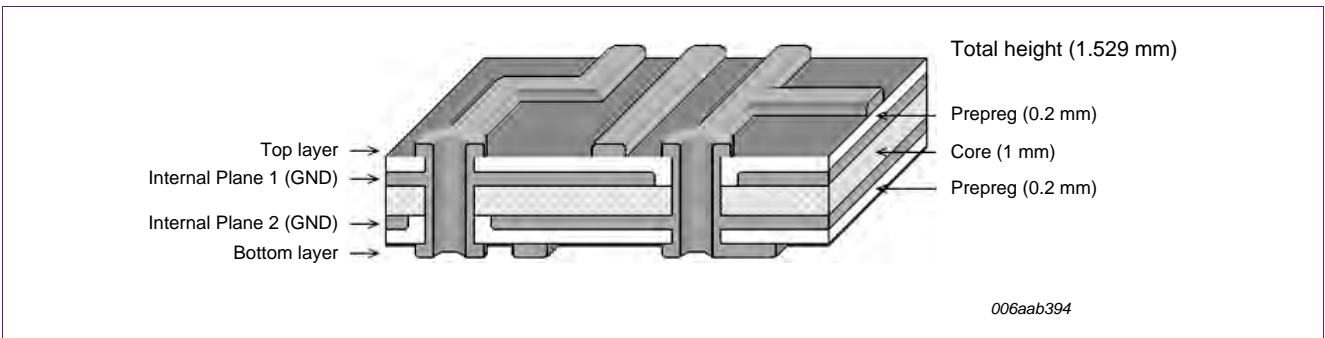
Fig 9. USB 2.0 PCB layer structure
