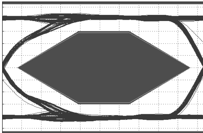
Fig 24. USB 2.0 “eye pattern” with PRTR5V0U2F protection diode; PCB3
