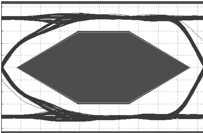
Fig 22. USB 2.0 “eye pattern” with PRTR5V0U2F protection diode; PCB1
