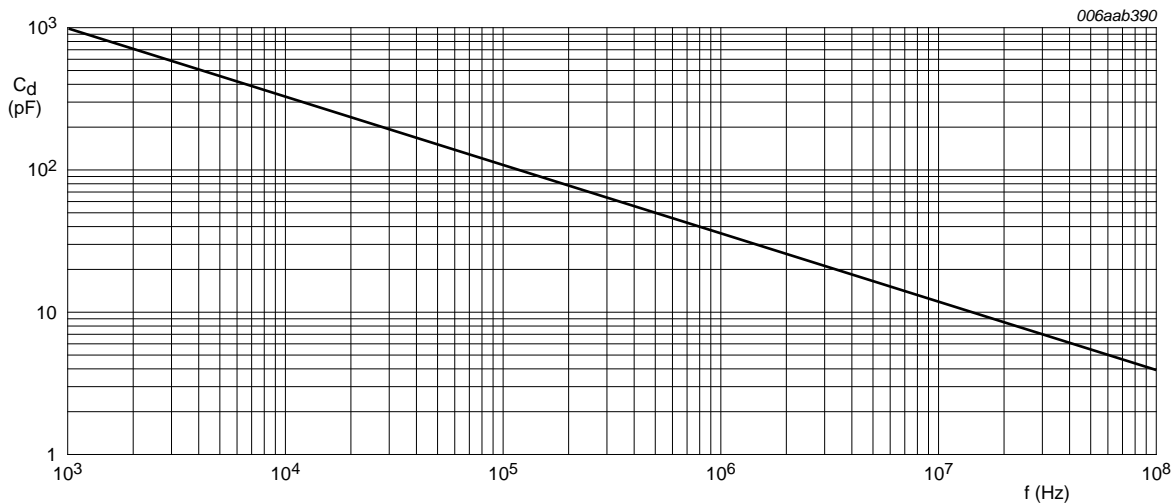
Fig 5. Line capacitance as a function of line frequency; typical values
