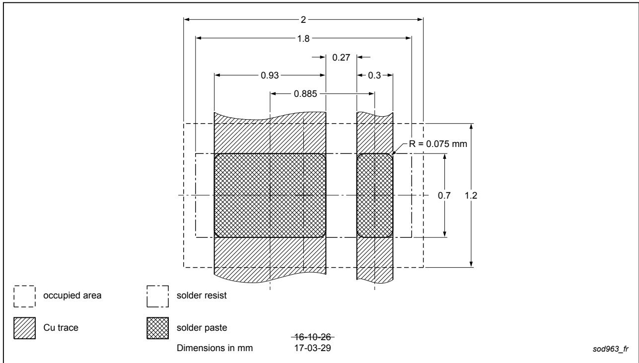
Fig. 2. Reflow soldering footprint for DSN1608-2 (SOD963)
