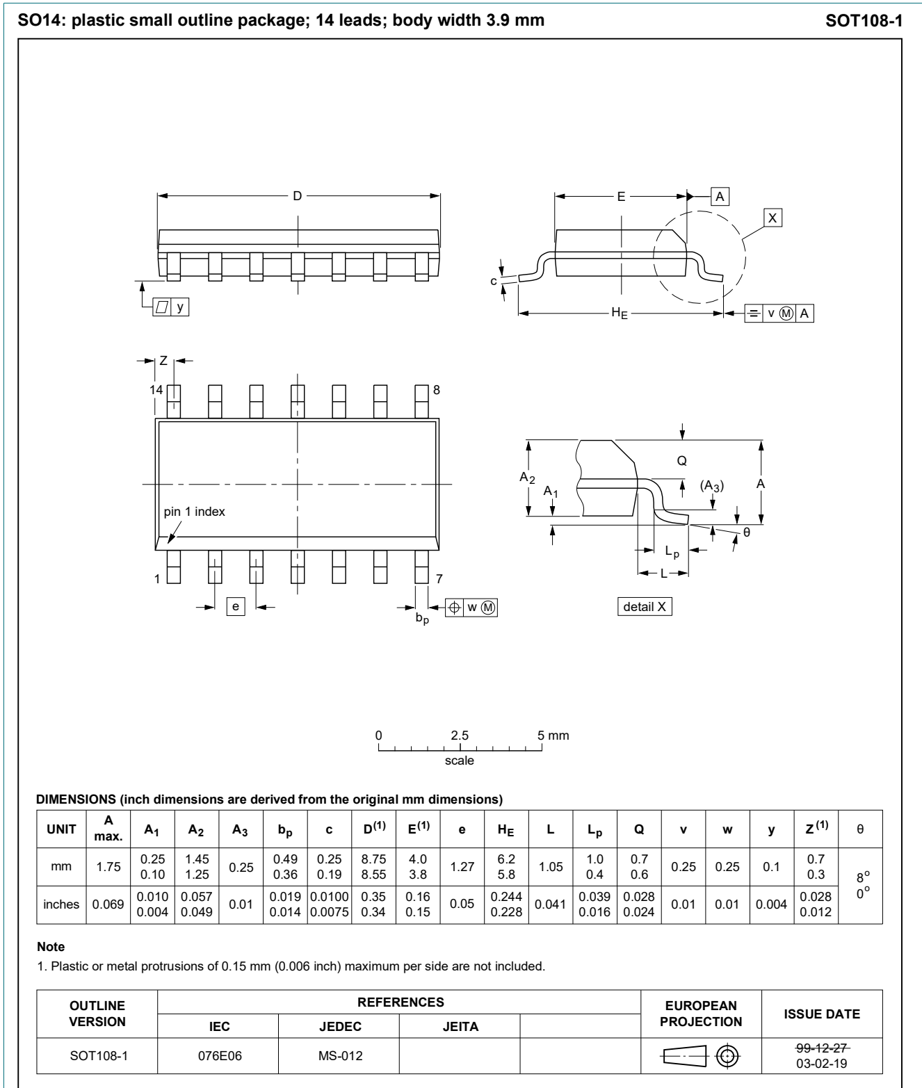
Fig. 1. Package outline SO14 (SOT108-1)
