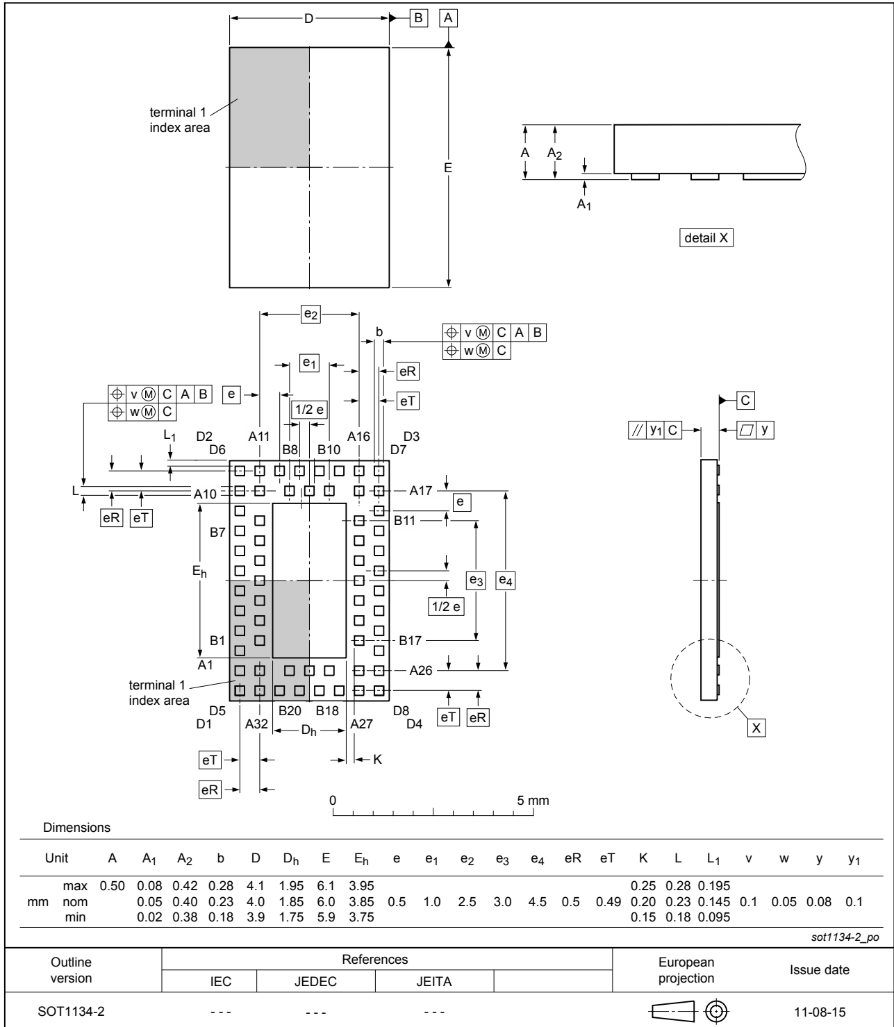
Fig. 1. Package outline HXQFN60U (SOT1134-2)
