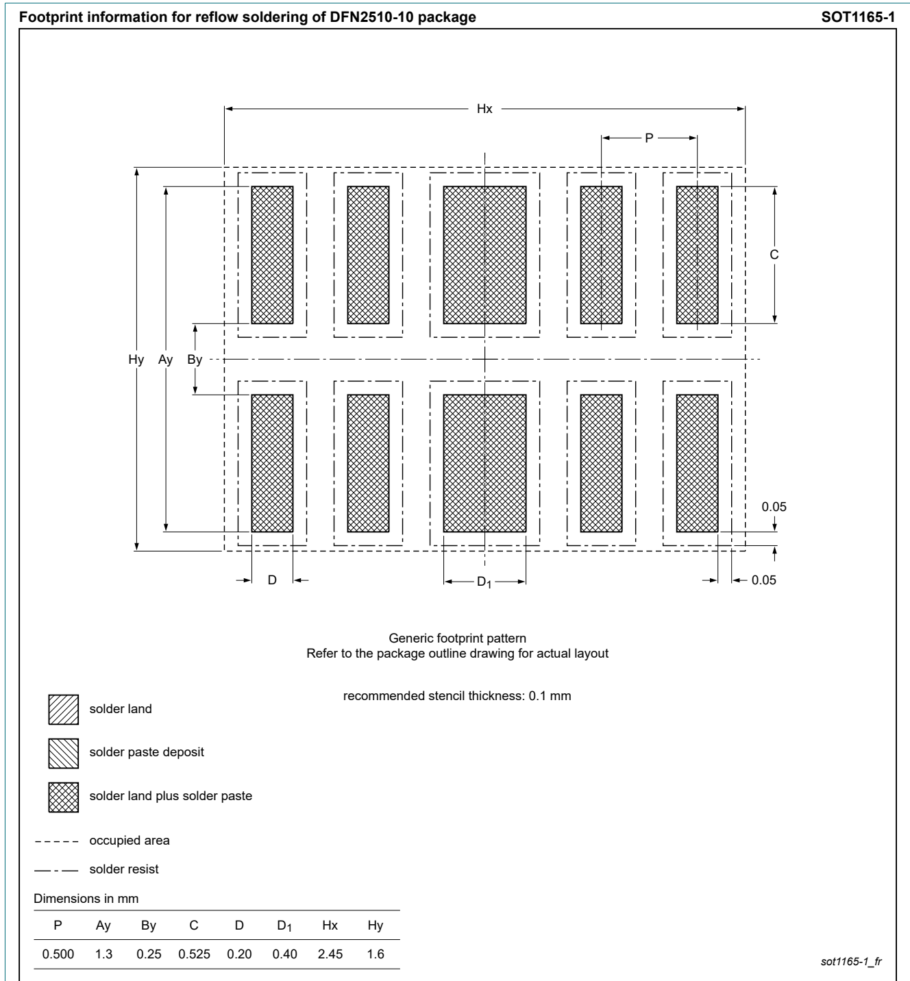
Fig. 2. Reflow soldering footprint for DFN2510-10 (SOT1165-1)
