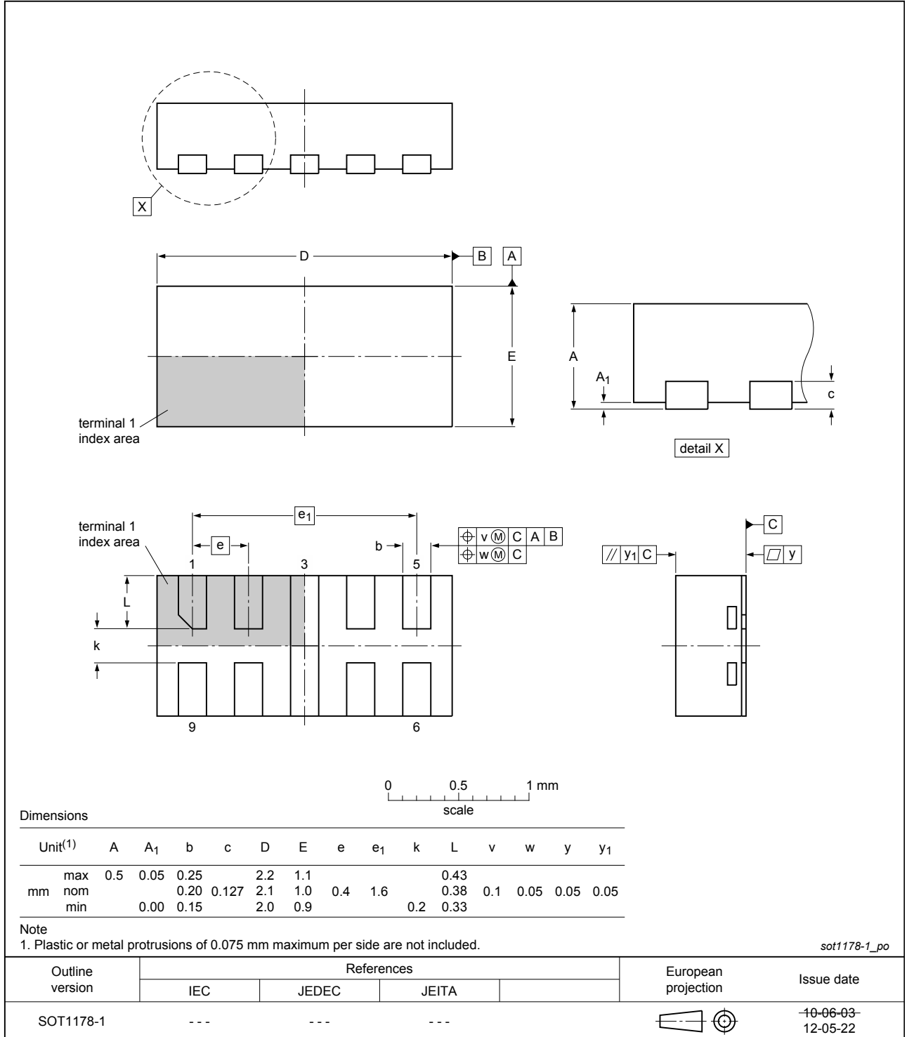
Fig. 1. Package outline DFN2110-9 (SOT1178-1)
