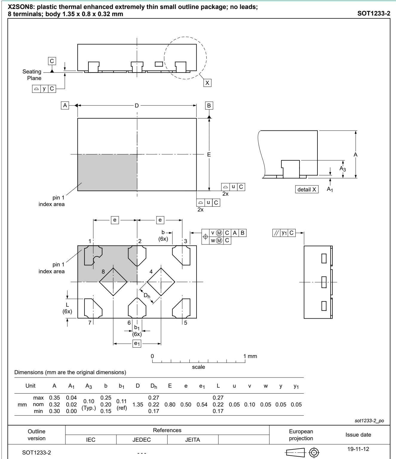
Fig. 1. Package outline X2SON8 (SOT1233-2)
