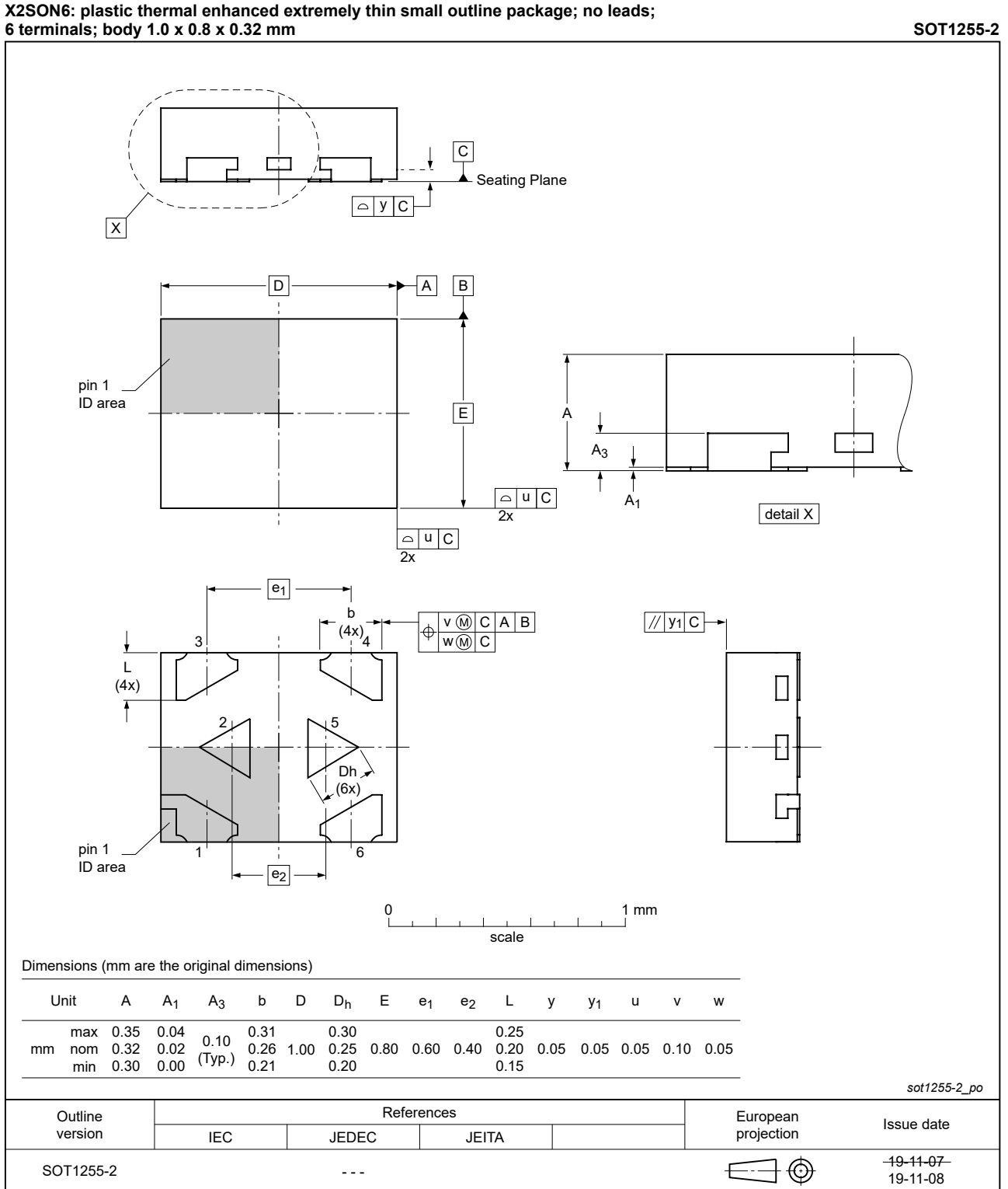
Fig. 1. Package outline X2SON6 (SOT1255-2)
