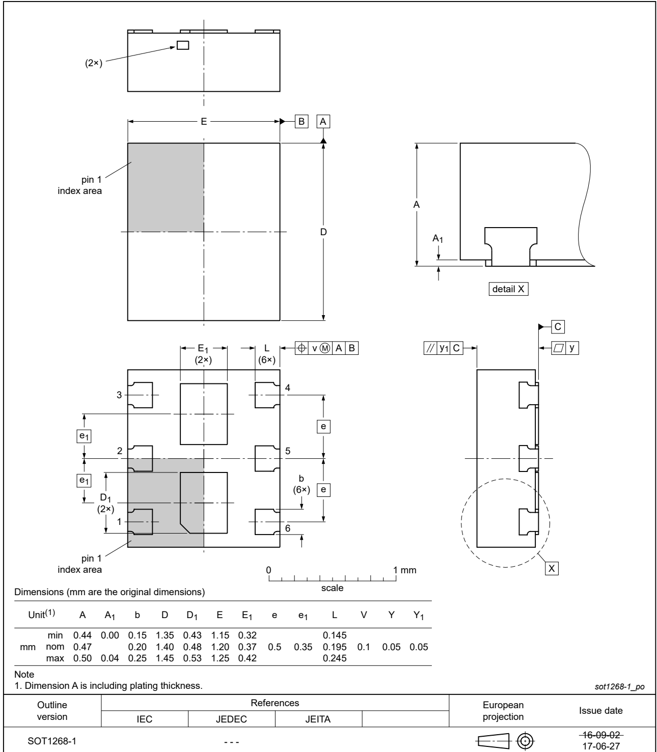
Fig. 1. Package outline DFN1412-6 (SOT1268-1)
