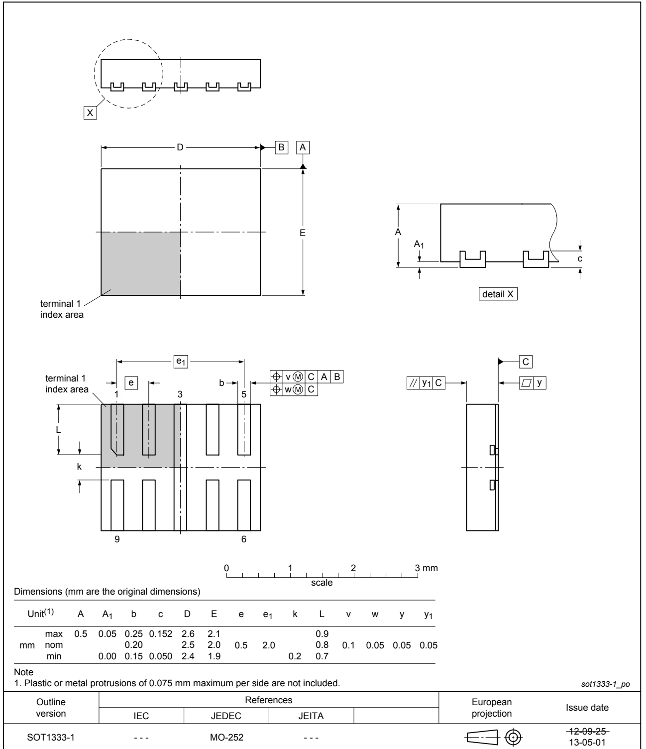
Fig. 1. Package outline XSON9 (SOT1333-1)
