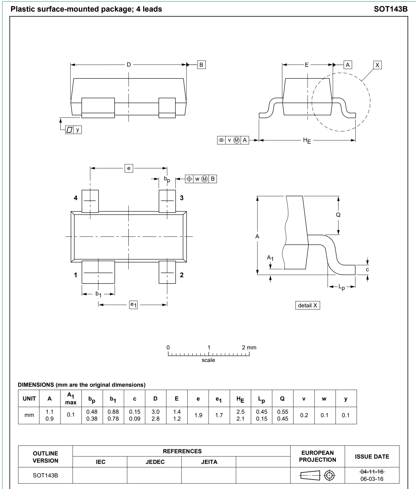
Fig. 1. Package outline SOT143B
