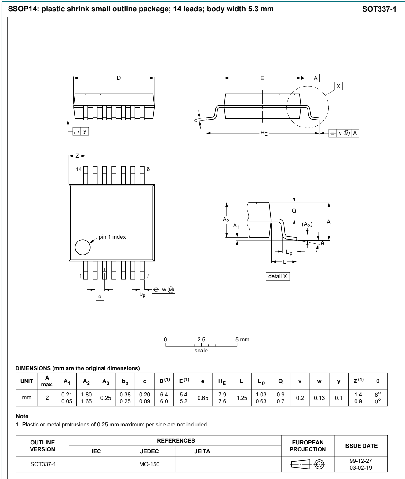
Fig. 1. Package outline SSOP14 (SOT337-1)
