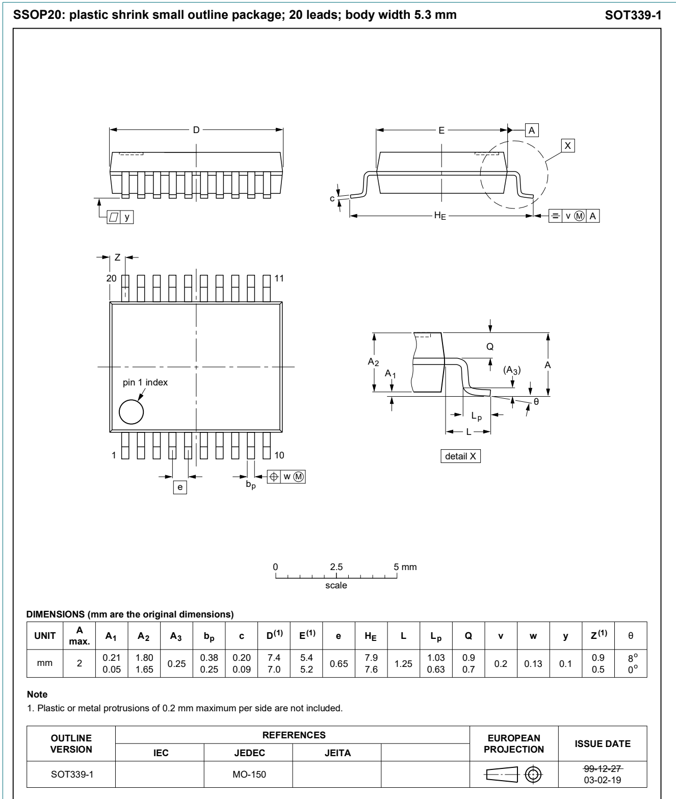
Fig. 1. Package outline SSOP20 (SOT339-1)
