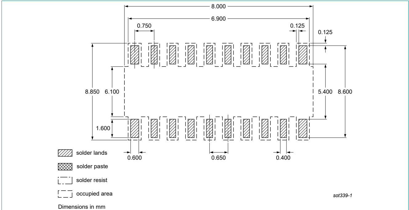
Fig. 2. Reflow soldering footprint for SSOP20 (SOT339-1)
