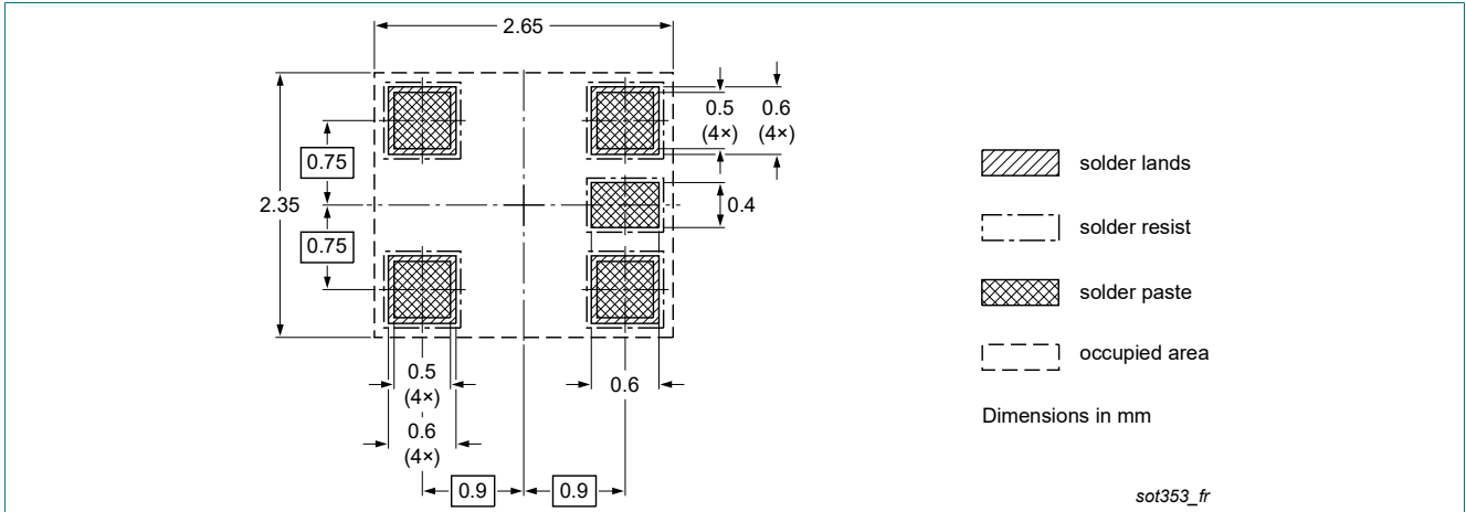
Fig. 2. Reflow soldering footprint for TSSOP5 (SOT353)
