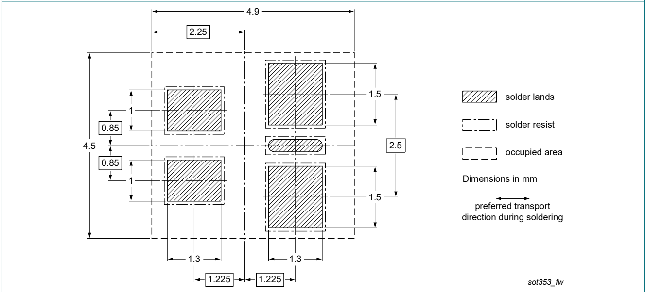
Fig. 3. Wave soldering footprint for TSSOP5 (SOT353)
