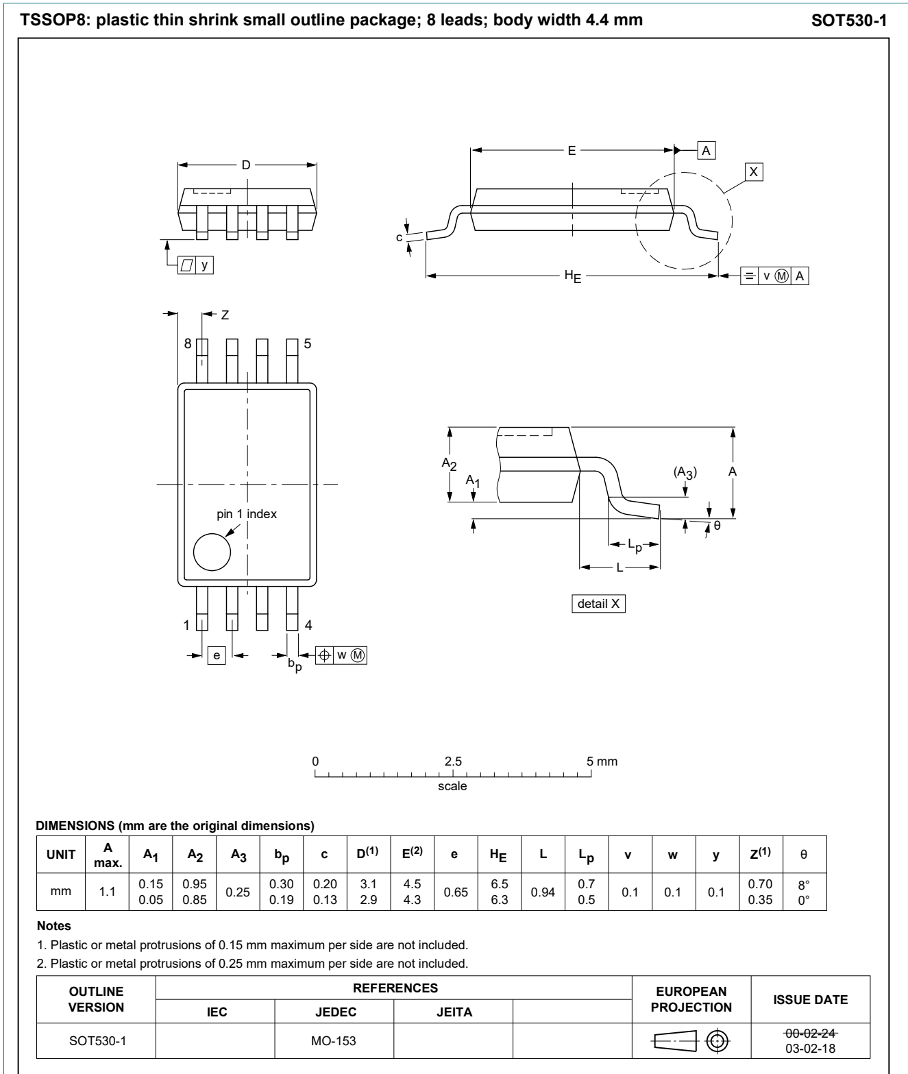
Fig. 1. Package outline TSSOP8 (SOT530-1)
