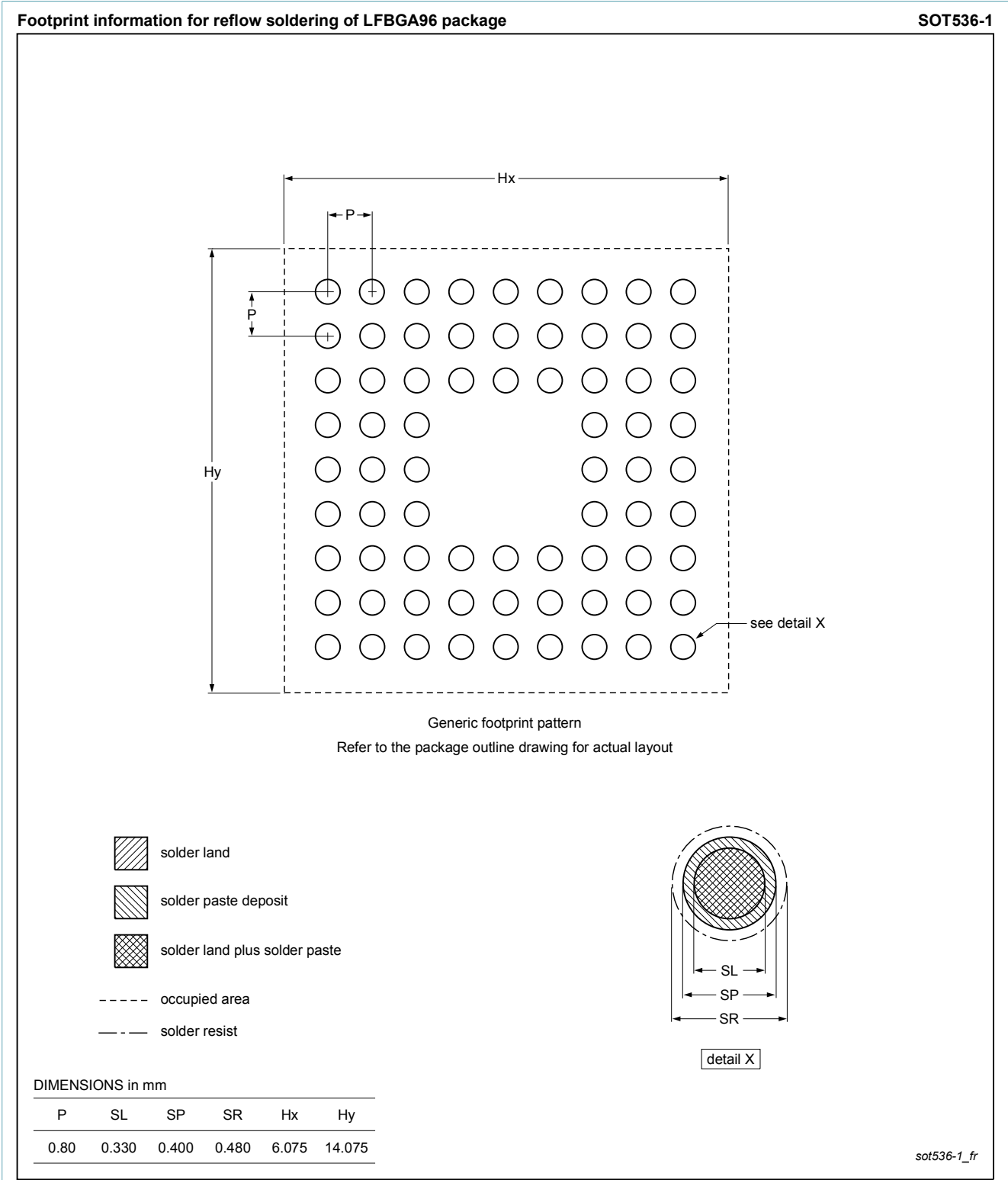
Fig. 2. Reflow soldering footprint for LFBGA96 (SOT536-1)
