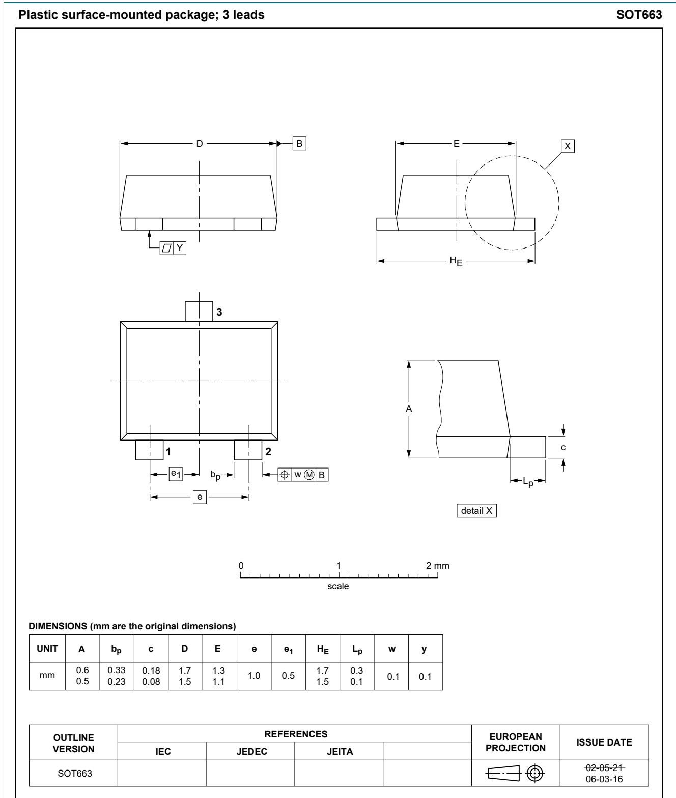
Fig. 1. Package outline SOT663
