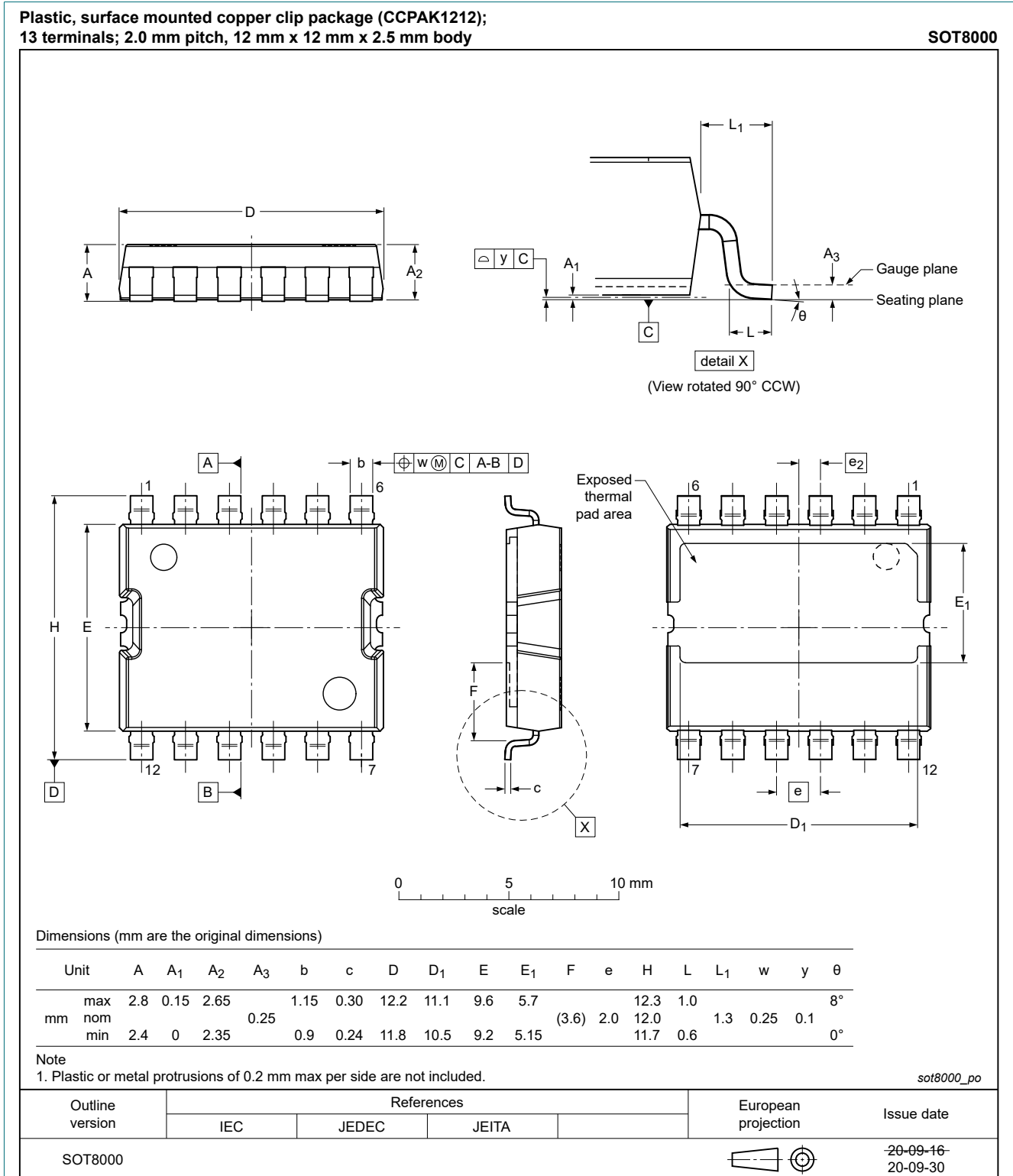
Fig. 1. Package outline CCPAK (SOT8000)
