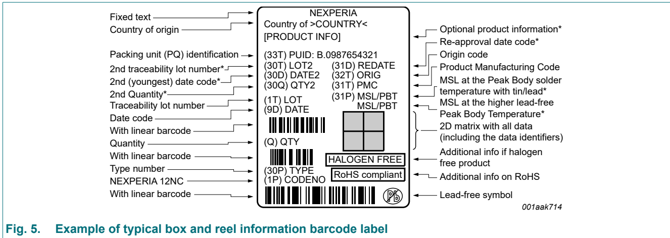
Fig. 5. Example of typical box and reel information barcode label
