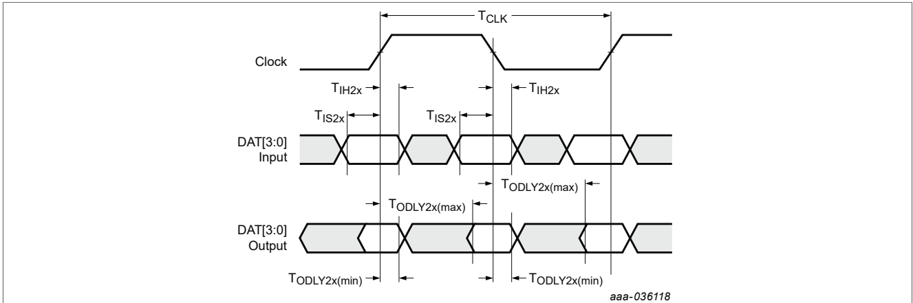
Figure 18. SDIO DAT[3:0] timing diagram—DDR50 mode [1] (50 MHz)
