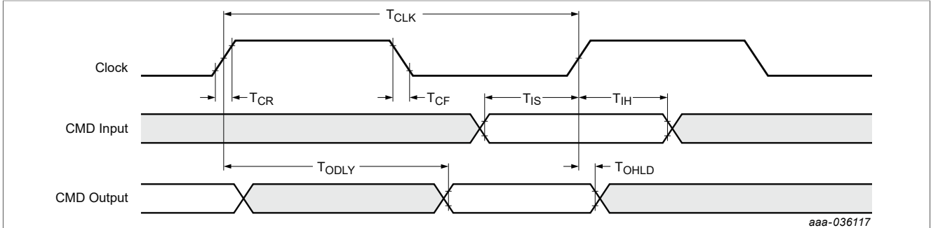
Figure 17. SDIO CMD timing diagram—DDR50 mode (50 MHz)
