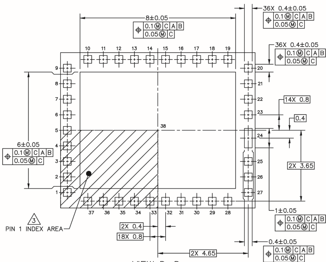
VIEW D-D (BOTTOM VIEW)
