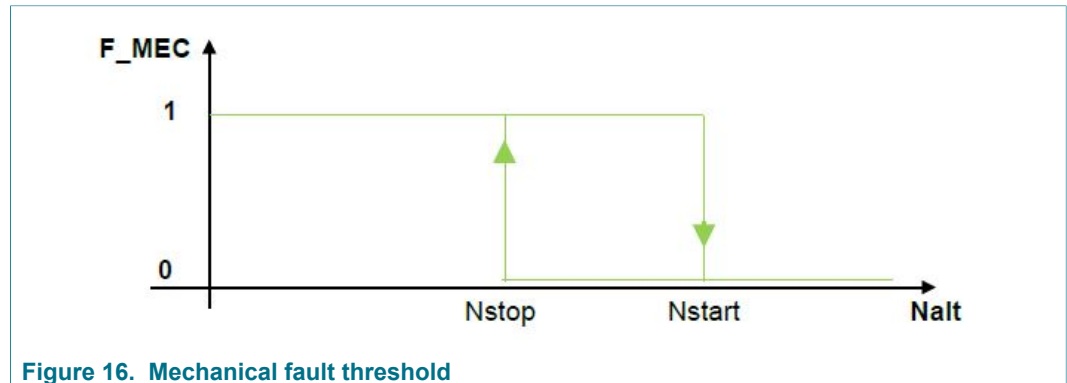
Figure 16. Mechanical fault threshold
