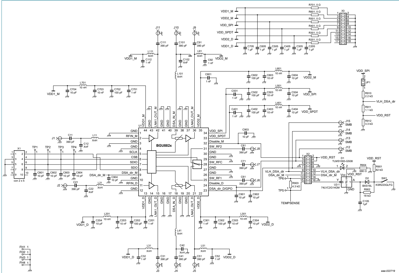
Figure 52. BGU8822/A application diagram.
