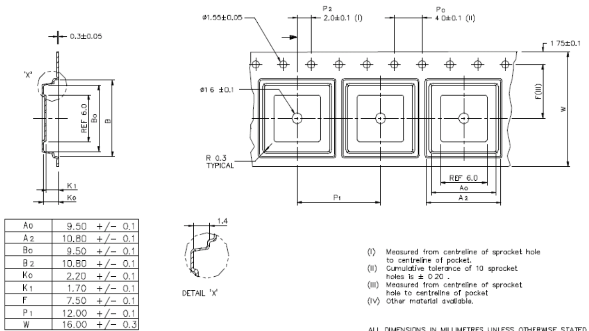
Figure 12. Tape package
