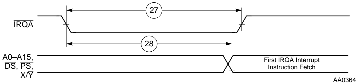
Figure 2-11 Recovery from Stop State Using IRQA Interrupt Service
