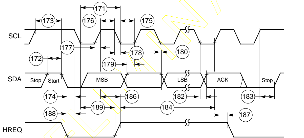
Figure 2-19 I 2 C Timing
