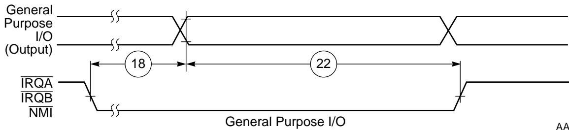
Figure 4-5. External Level-Sensitive Fast Interrupt Timing
