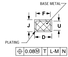
SECTION AB-AB ROTATED 90 CLOCKWISE
