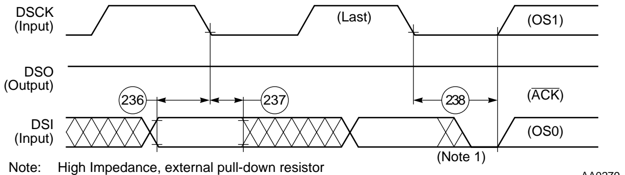
Figure 4-24. DSP56012 OnCE Data I/O to Status Timing
