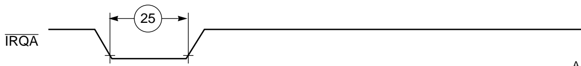
Figure 4-6. Recovery from Stop State Using \overline{IRQA}
