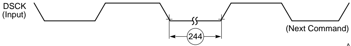
Figure 4-28. DSP56012 OnCE DSK Next Command After Read Register Timing
