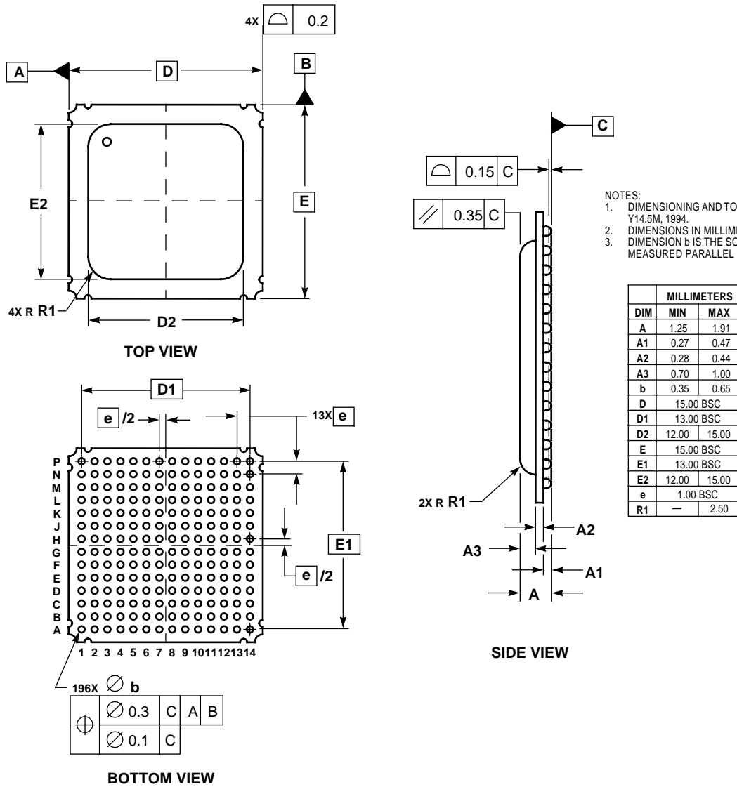
Figure 3-3 DSP56307 Mechanical Information, 196-pin PBGA Package
