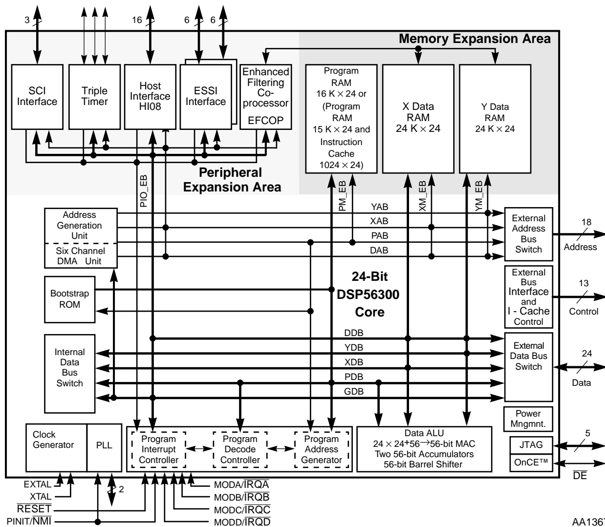
Figure 1 DSP56307 Block Diagram
