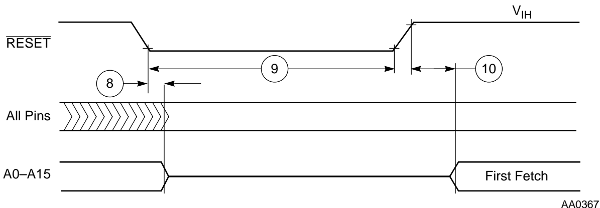
Figure 2-3 Reset Timing
