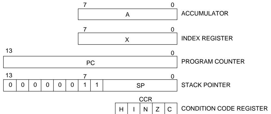
Figure 3-1. Programming Model
