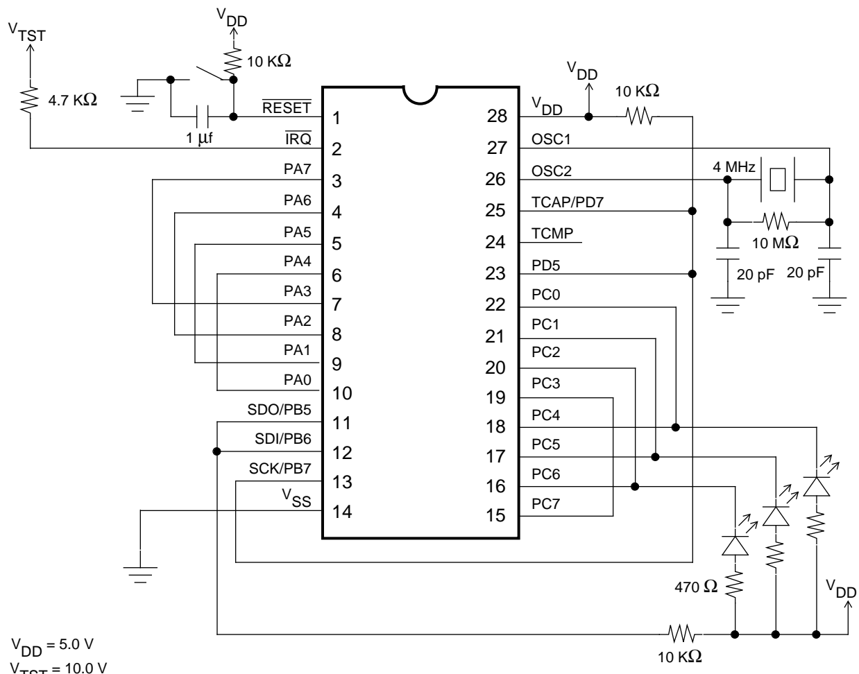
Figure 10-1. Self-Check Circuit
