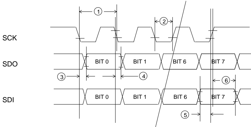
Figure 12-1. SIOPIF Timing Diagram
