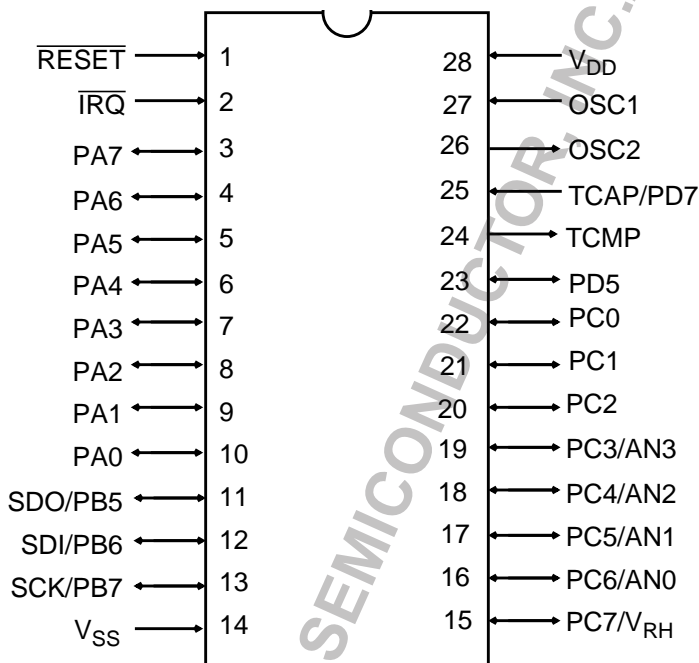
Figure 1-2. Pin Assignments
