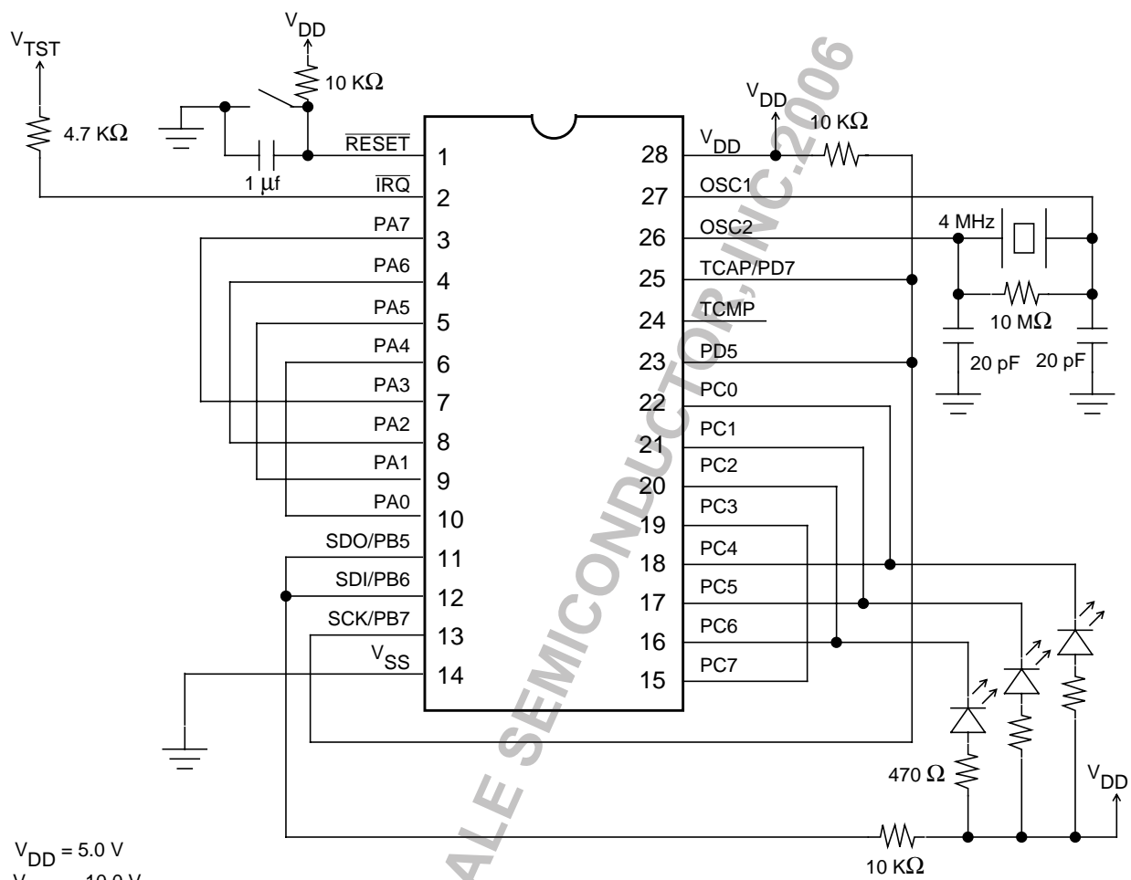
Figure 11-1. Self-Check Circuit
