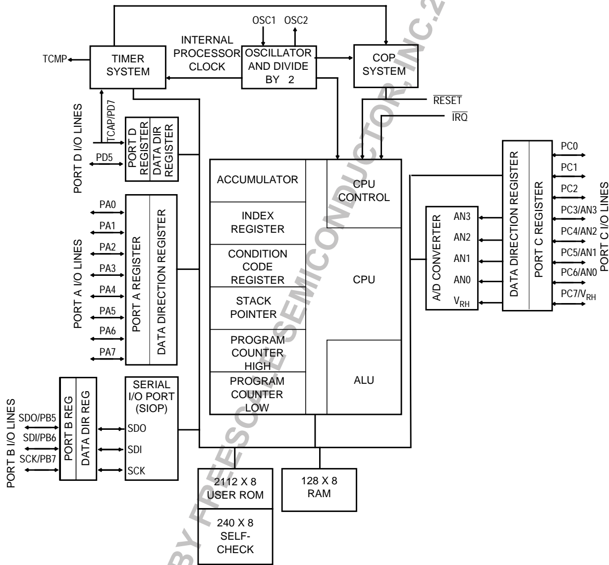
Figure 1-1. Block Diagram
