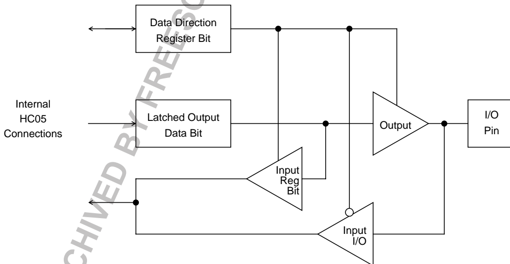
Figure 1-4. I/O Circuitry
