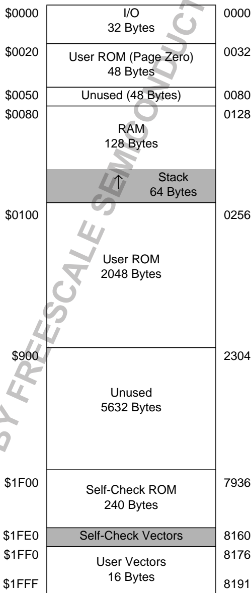
Figure 2-1. Memory Map
