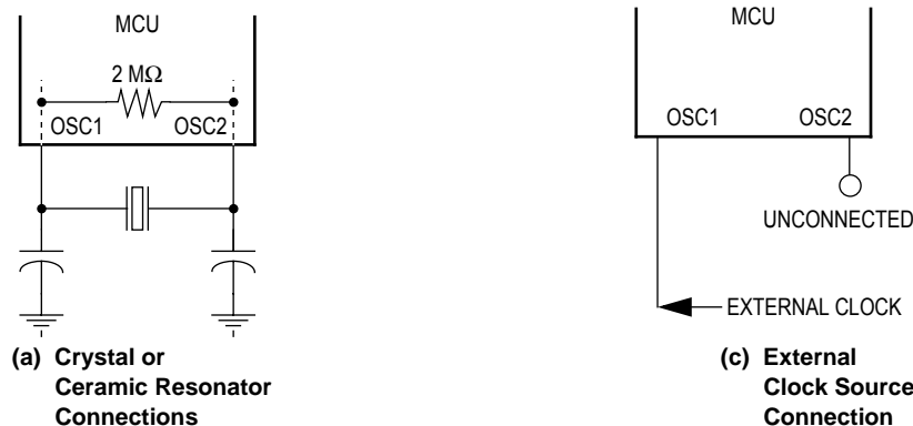
Figure 1-4. Oscillator Connections
