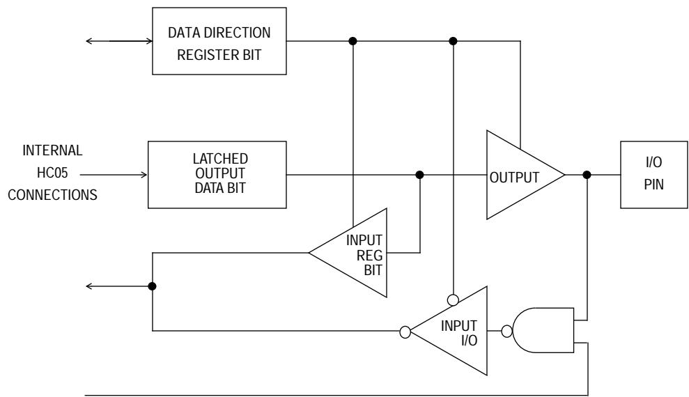
Figure 7-2. I/O Circuitry
