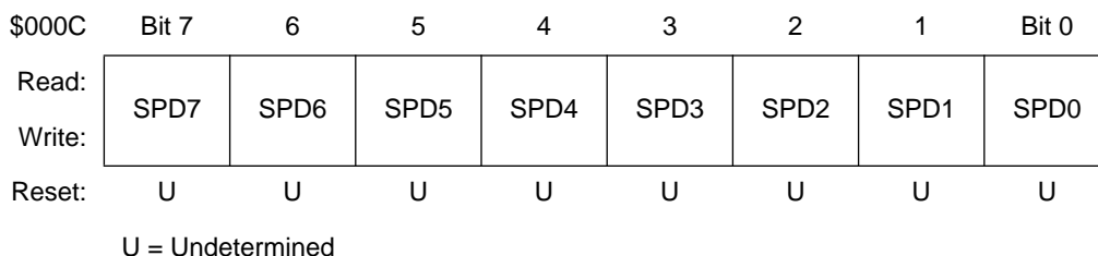
Figure 10-6. PI Data Register (SPDR)
