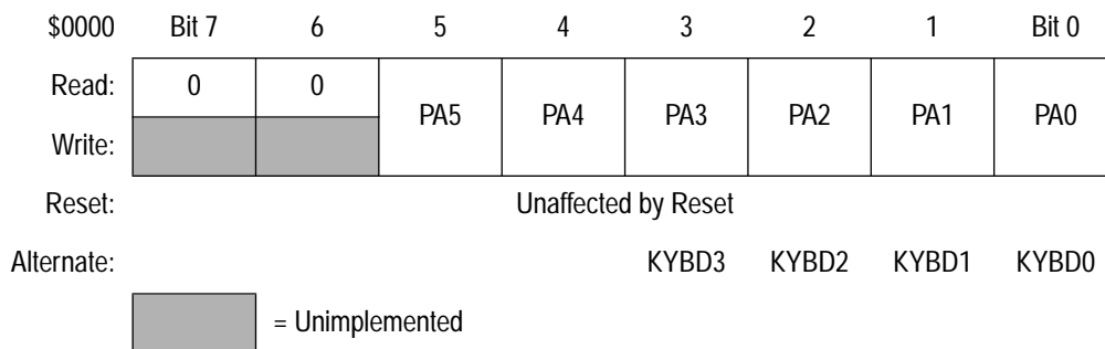
Figure 7-1. Port A Data Register (PORTA)
