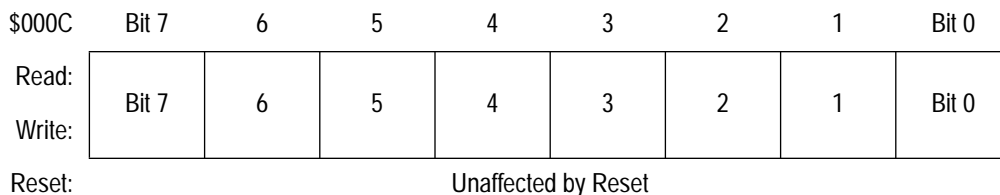
Figure 9-6. SIOPI Data Register (SDR)
