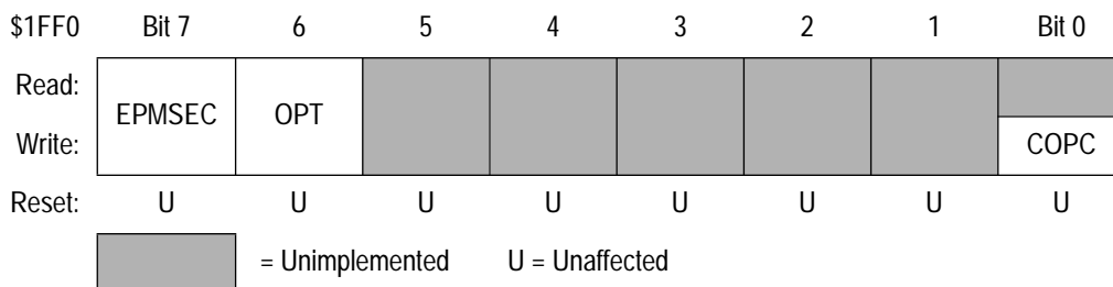
Figure 5-2. COP and Security Register (COPR)
