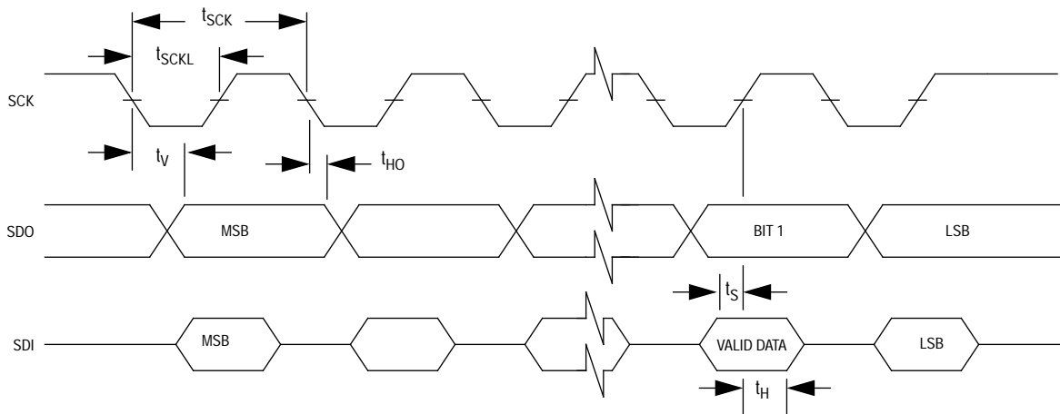
Figure 15-1. SIOPI Timing Diagram
