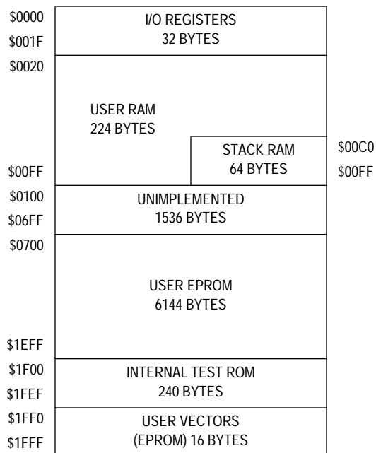
Figure 2-1. Memory Map
