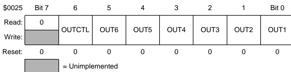
Figure 9-28. PWM Output Control Register (PWMMOUT)
