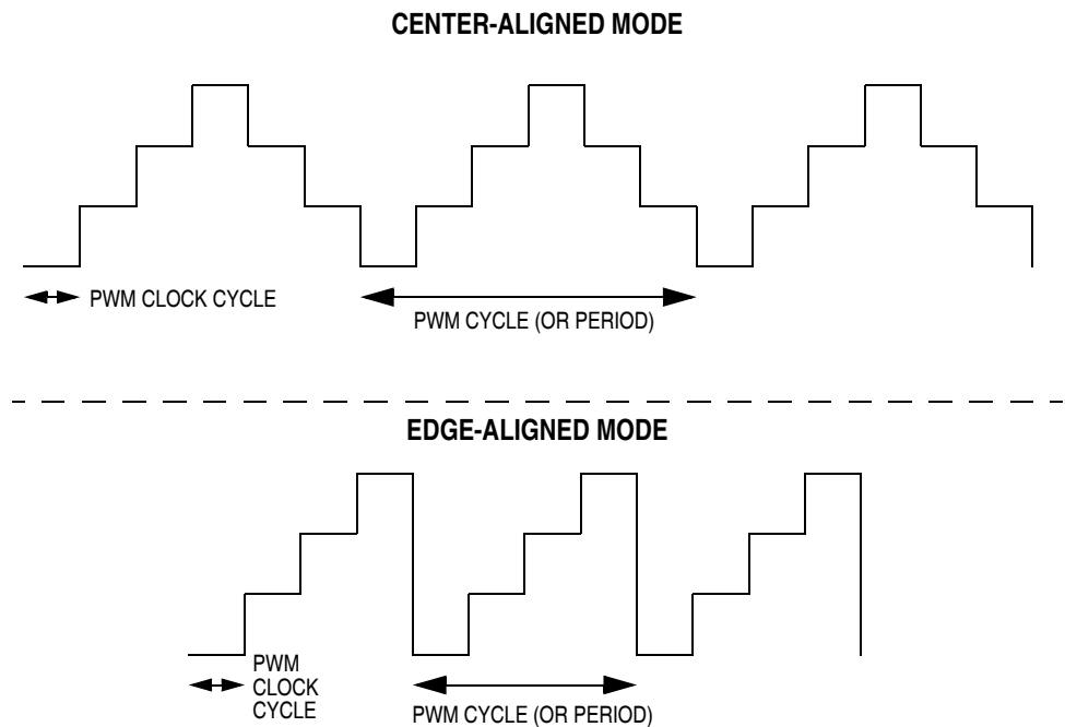
Figure 9-51. PWM Clock Cycle and PWM Cycle Definitions
