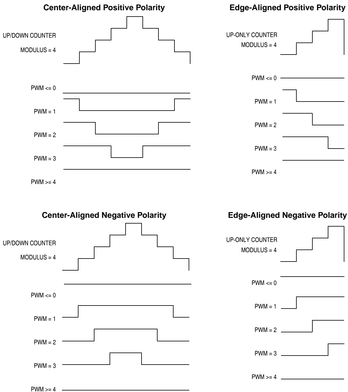
Figure 9-27. PWM Polarity
