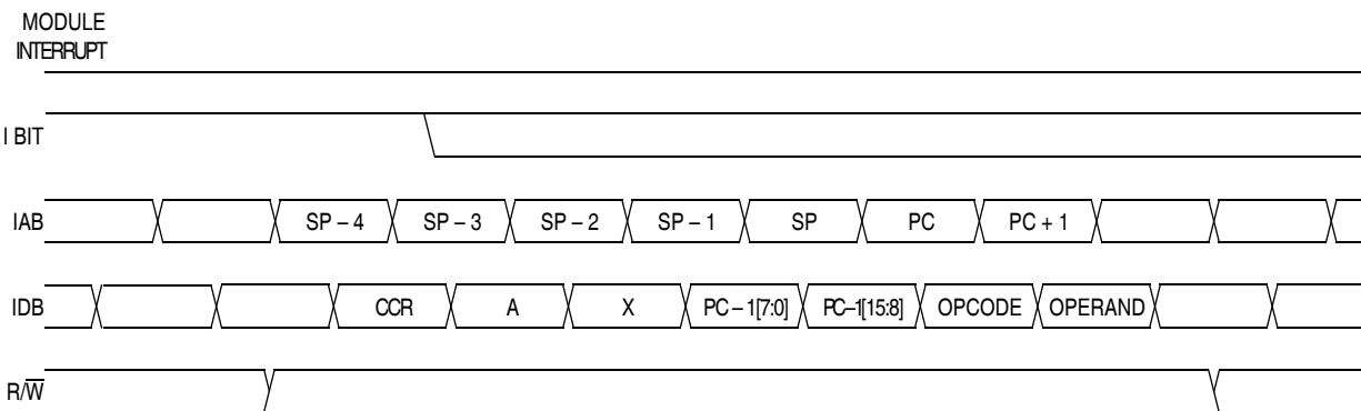
Figure 7-10. Interrupt Recovery
