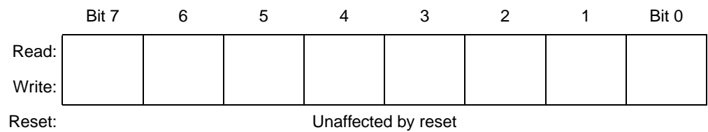
Figure 6-2. Accumulator (A)
