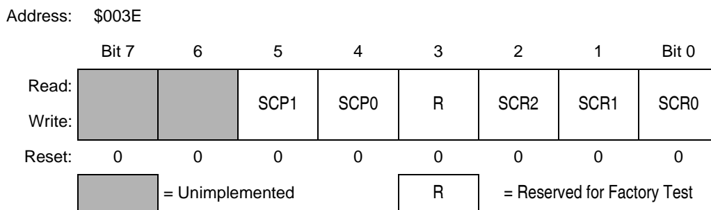
Figure 14-14. SCI Baud Rate Register (SCBR)
