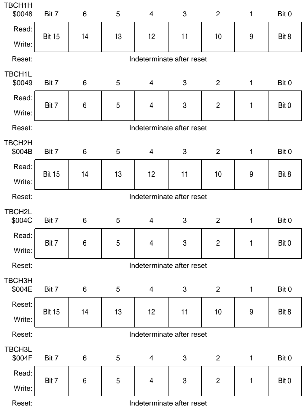
Figure 12-9. TIMB Channel Registers (TBCH0H/L:TBCH3H/L) (Continued)
