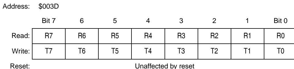
Figure 14-13. SCI Data Register (SCDR)
