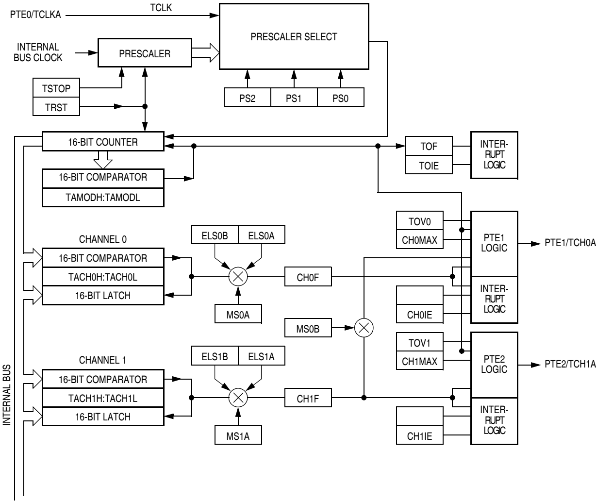
Figure 11-1. TIMA Block Diagram
