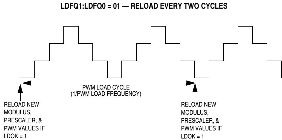
Figure 9-52. PWM Load Cycle/Frequency Definition
