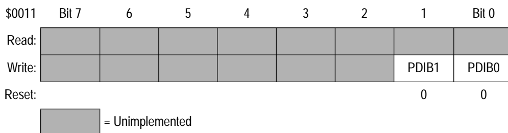
Figure 7-4. Port B Pulldown Inhibit Register (PDRB)
