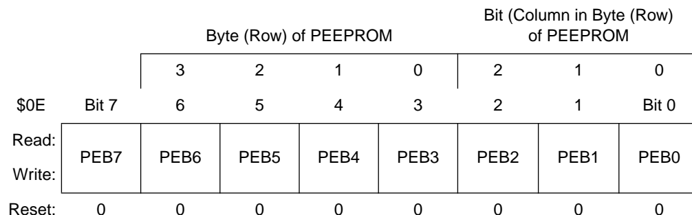
Figure 9-2. PEBSR Select Register
