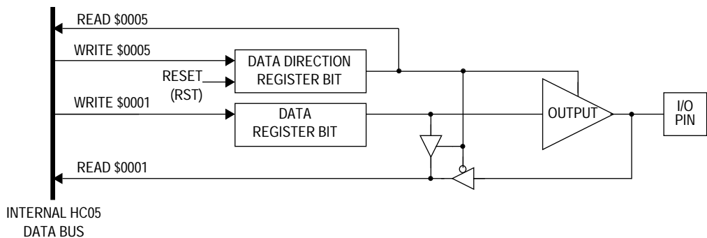
Figure 7-2. Port B I/O Circuitry
