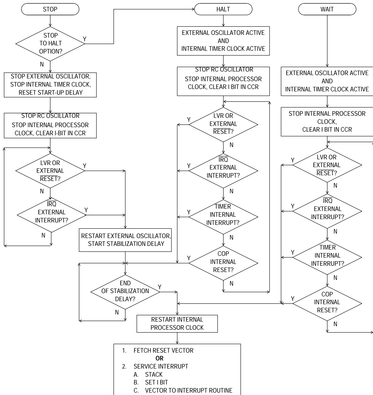
Figure 6-2. STOP/WAIT Flowcharts
