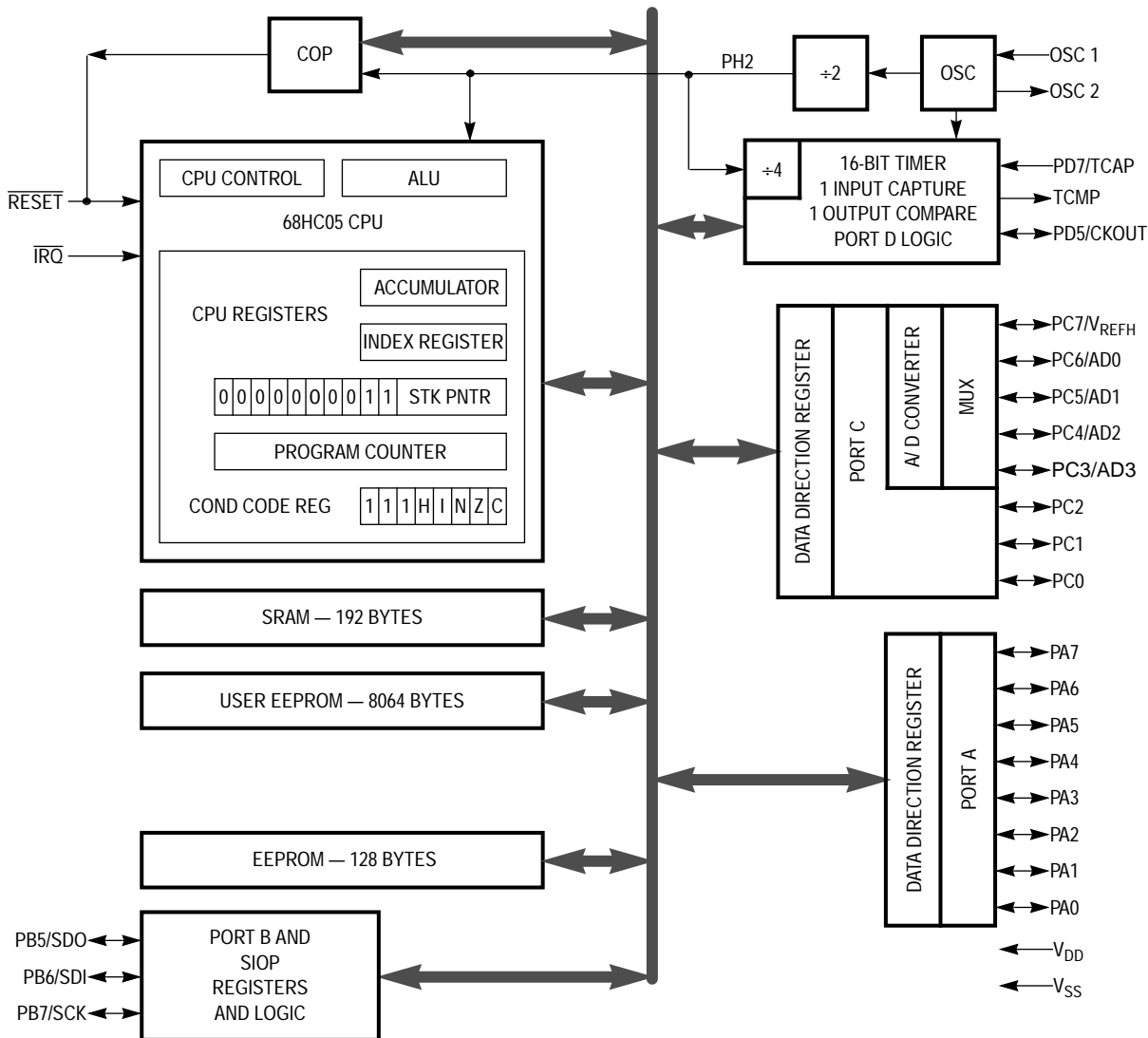
Figure 1-1. Block Diagram
