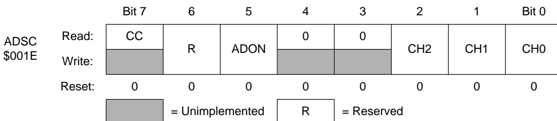
Figure 9-1. A/D Status and Control Register
