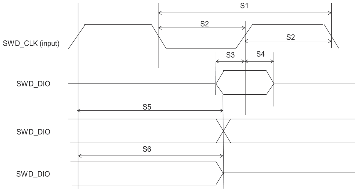
Figure 14. SWD timing
