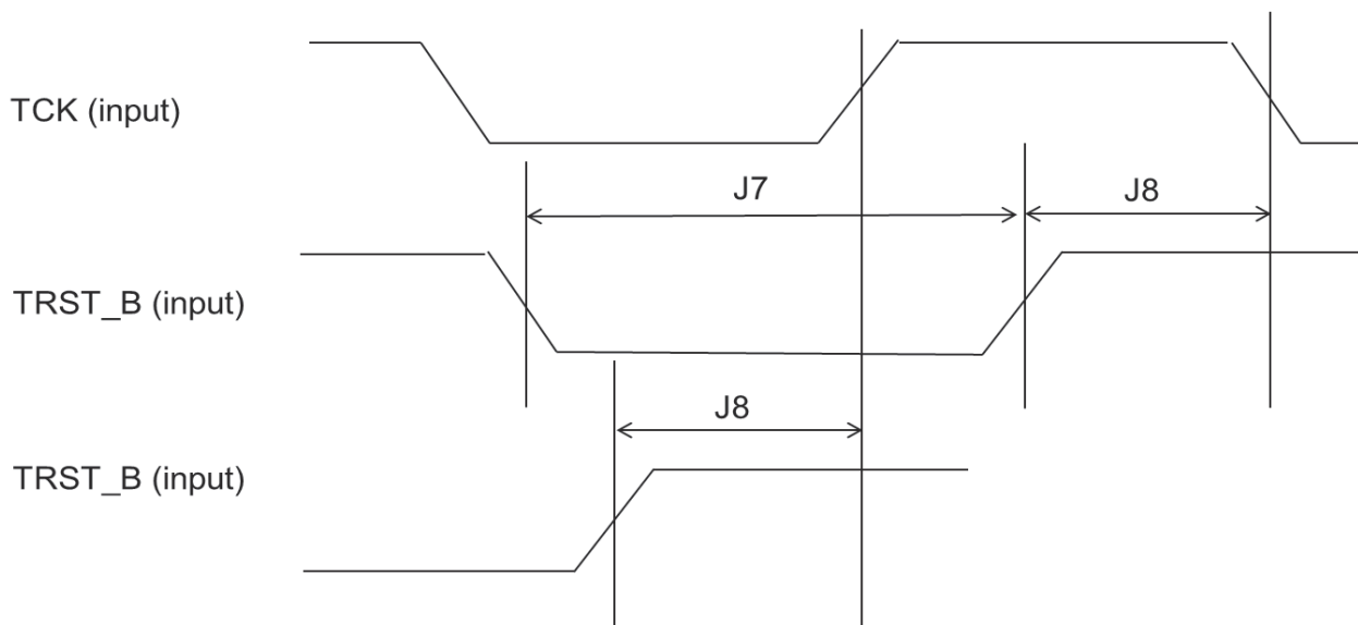
Figure 13. JTAG_TRST_B timing
