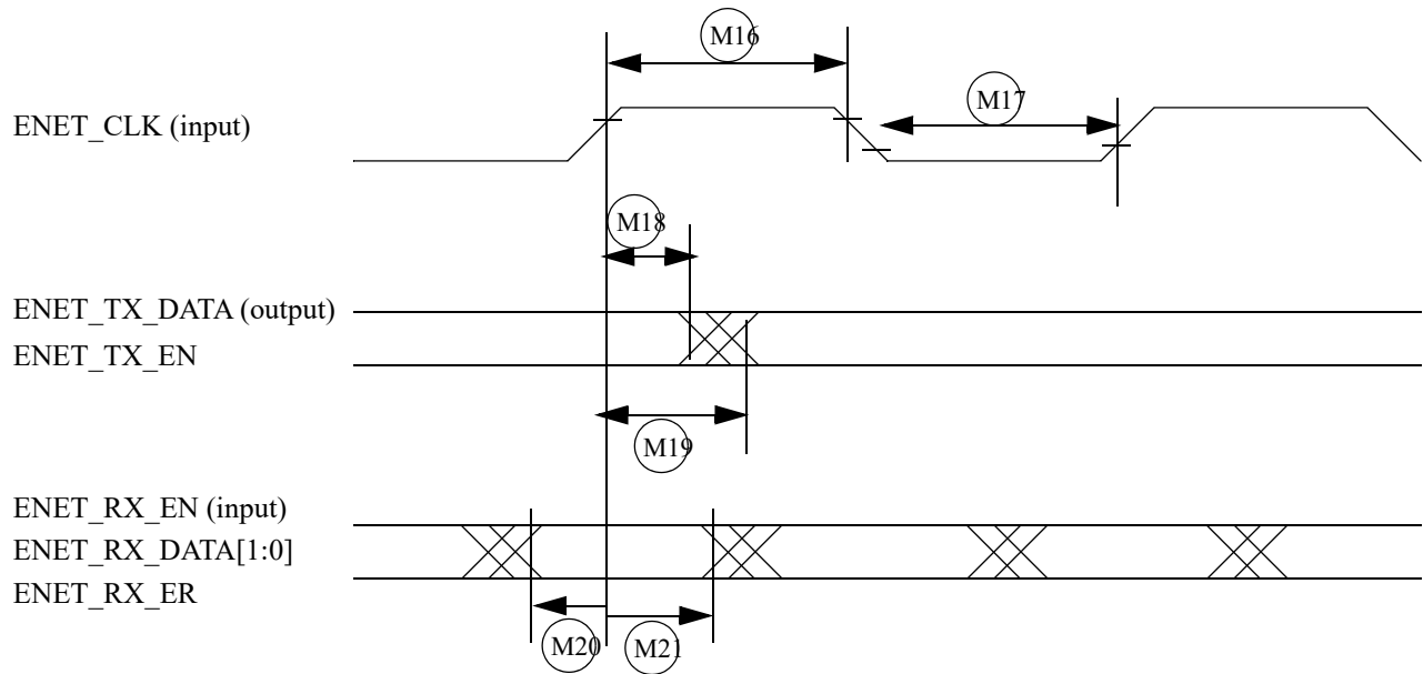
Figure 49. RMI mode signal timing diagram
