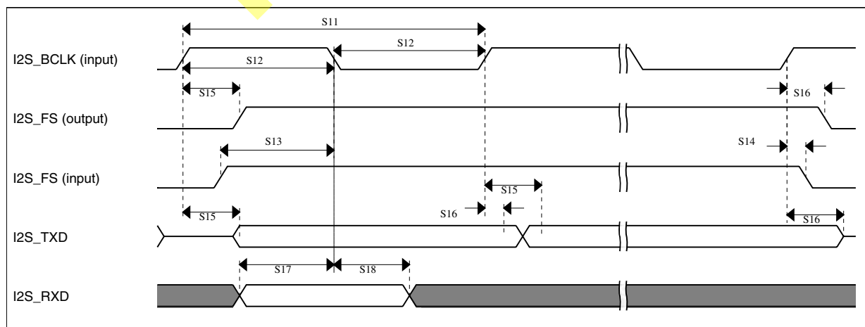
Figure 21. I 2 S timing — slave modes
